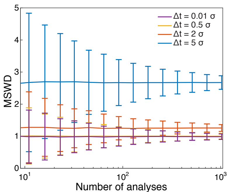
Figure S-4 The uncertainty of the MSWD for analytical datasets as a function of N for a range of \Delta t/\sigma . The case of \Delta t = 5\sigma is not distinguishable from instantaneous crystallisation with N less than \sim 50 , and \Delta t = 2\sigma is not distinguishable with N less than \sim 700 .
