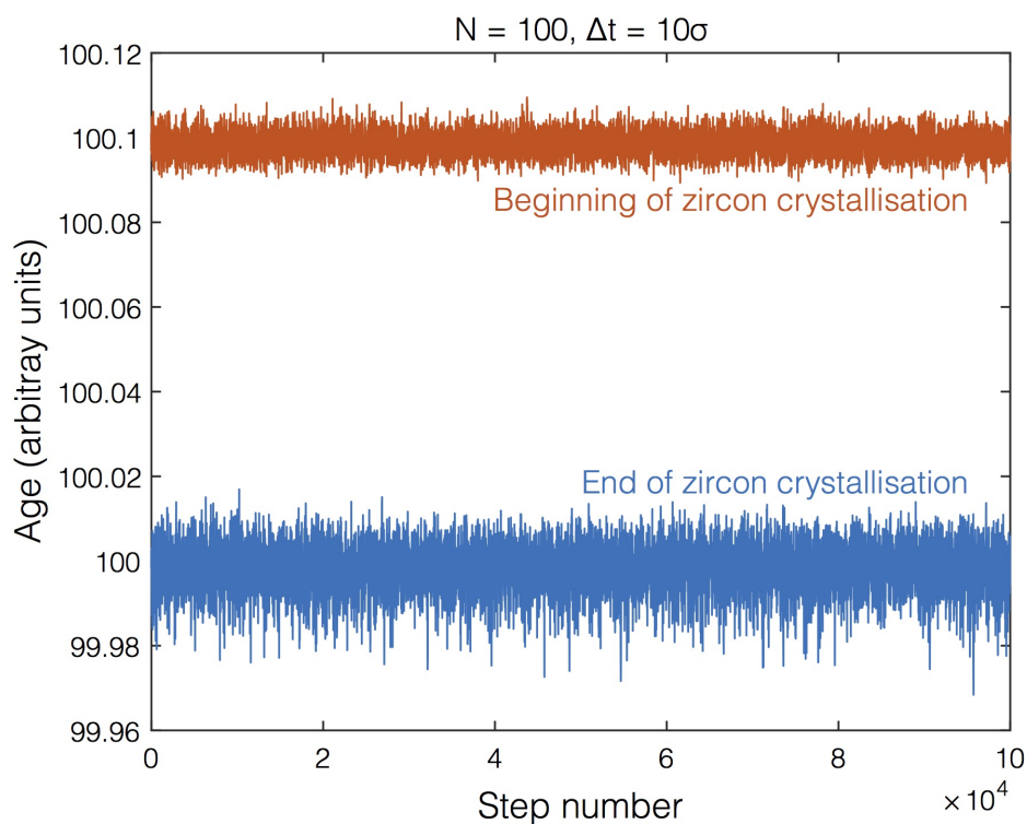
Figure S-3 Saturation and eruption ages of the first 10^5 steps of the Markov chain for an MCMC inversion of a synthetic dataset with 100 zircons and \Delta t = 10\sigma . Due to the simple monotonic nature of the likelihood function for such an age inversion, and the availability of accurate initial guesses (i.e., the oldest and youngest zircon), the distribution is immediately stationary. A weighted mean age must always plot on the line of instantaneous crystallisation.
