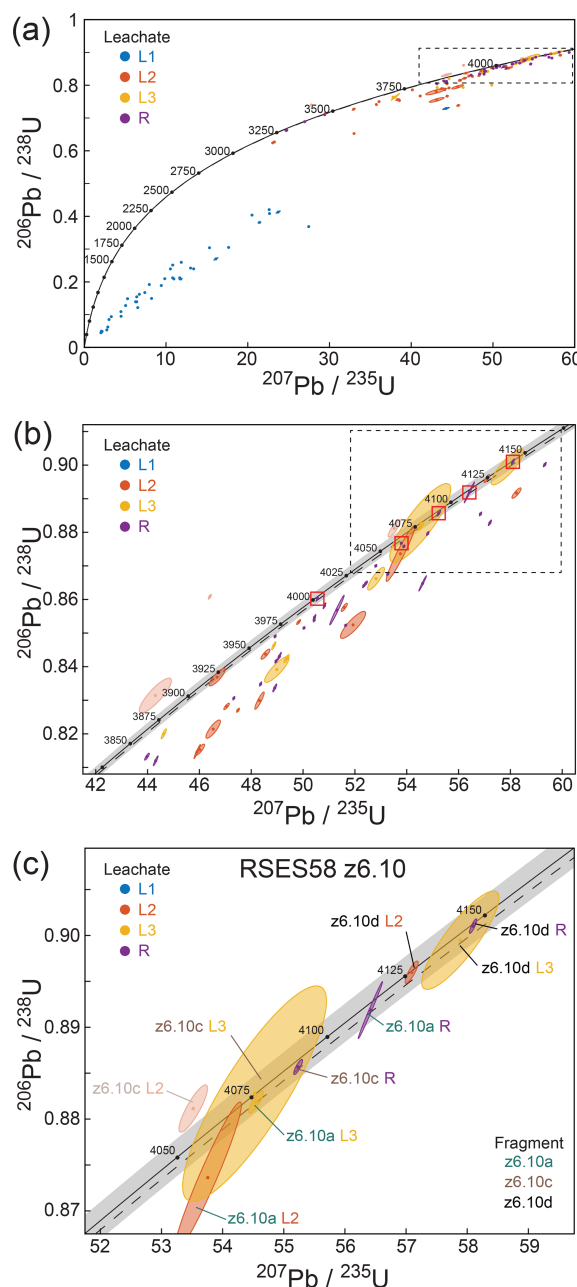
Figure 2. CA-ID-TIMS ages for Jack Hills zircon by fragment and leaching step in Wetherill (1956) concordia space. (a) Full range, including recent Pb-loss array in L1 leachates. (b) Hadean–Eoarchean inset, emphasizing the complexity of the Hadean record and suggesting early lead loss and protracted crystallization history. Concordant residues are highlighted with red squares. (c) Concordant fragments and leachates of zircon RSES58 z6.10, illustrating \sim 50 Myr age heterogeneity between concordant residues of zircon fragments from the same polished half-zircon. At this scale, the uncertainty in the \lambda_{\text{U-238}}/\lambda_{\text{U-235}} decay constant ratio that defines concordia becomes important; here the solid concordia line and grey two-sigma error envelope reflect the values of Jaffey et al. (1971), while the dashed line reflects those of Schoene et al. (2006). All dates plotted along the concordia line are in millions of years.
